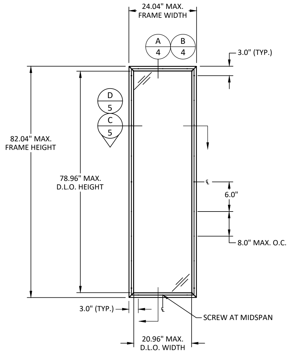
ELEVATION KEYSTONE FRAME
