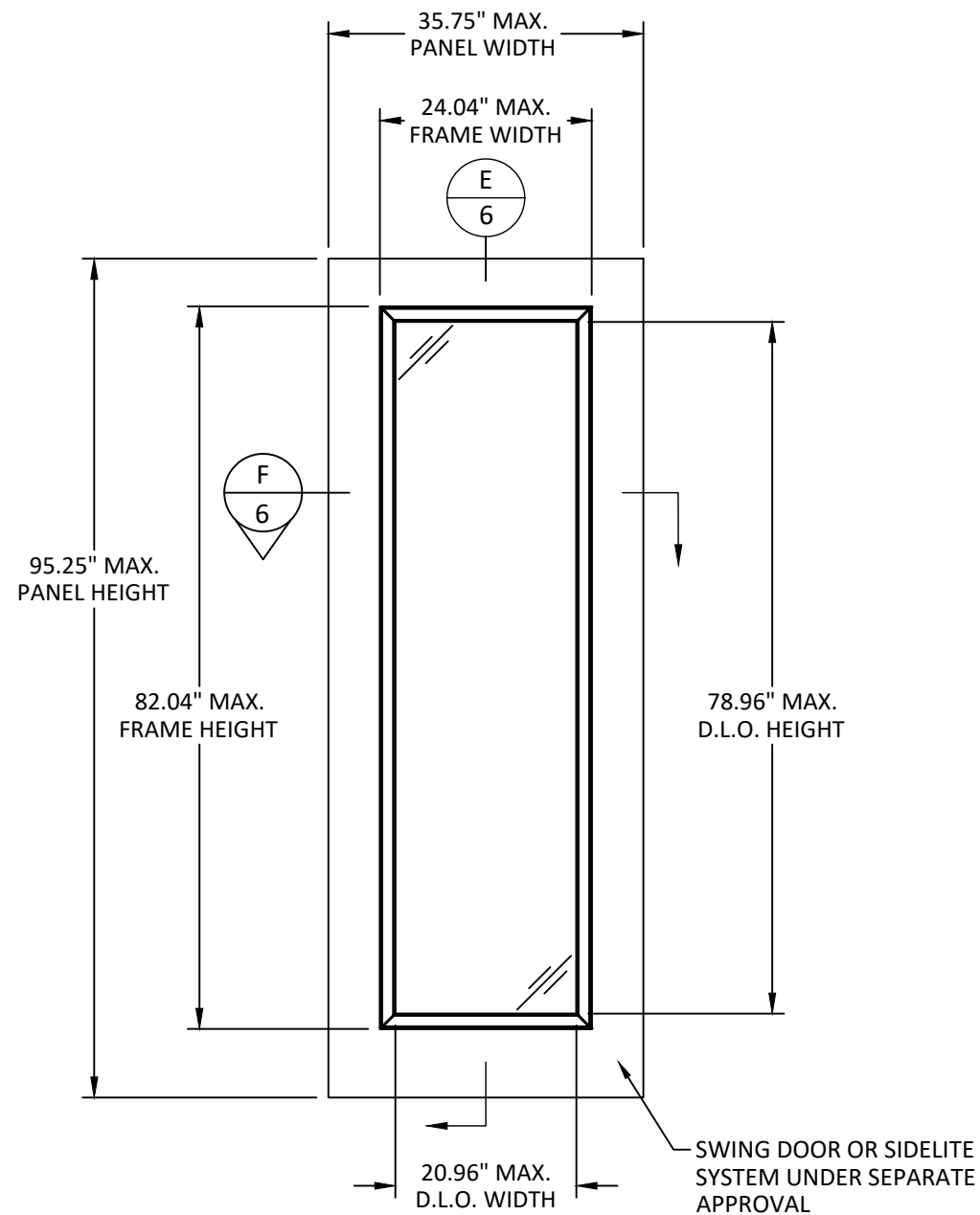
ELEVATION PLASTPRO 8'-0" PANEL
