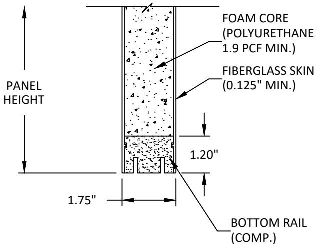
E 6 VERTICAL SECTION PLASTPRO PANEL
